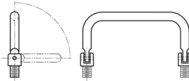
Round - 90° 2 Position - External Thread
