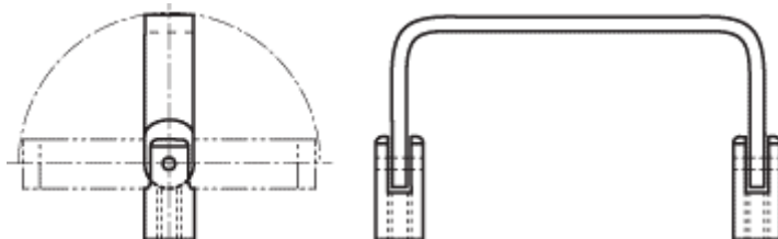
Rectangle – 180° Infinite Position Internal Thread
