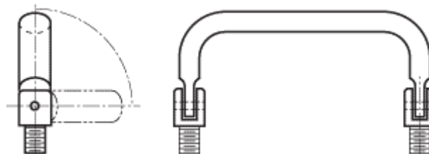
Oval - 90° 2 Position - External Thread
