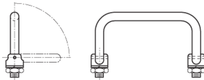
Round - 90° Free Fall – External Thread
